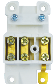
HYJB43TE (Inside view showing Earth Tab)
