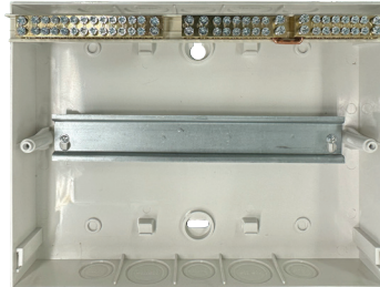
NEUTRAL LINK RATING: 100A
