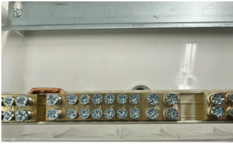
100A RATED ASSEMBLY
