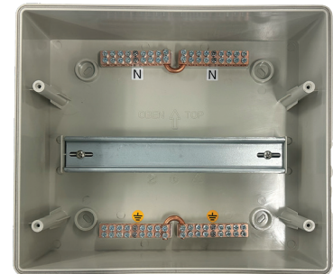
100A RATED ASSEMBLY WITH NEUTRAL & EARTH BARS
