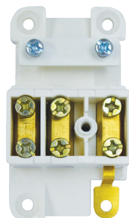
HYJB3TE (Inside view showing Earth Tab)
