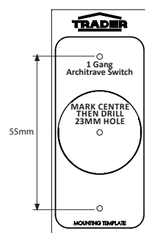
example of cutting template COSWVA1G
