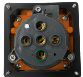
Size 2 Single/Three Phase 32A - 50A
